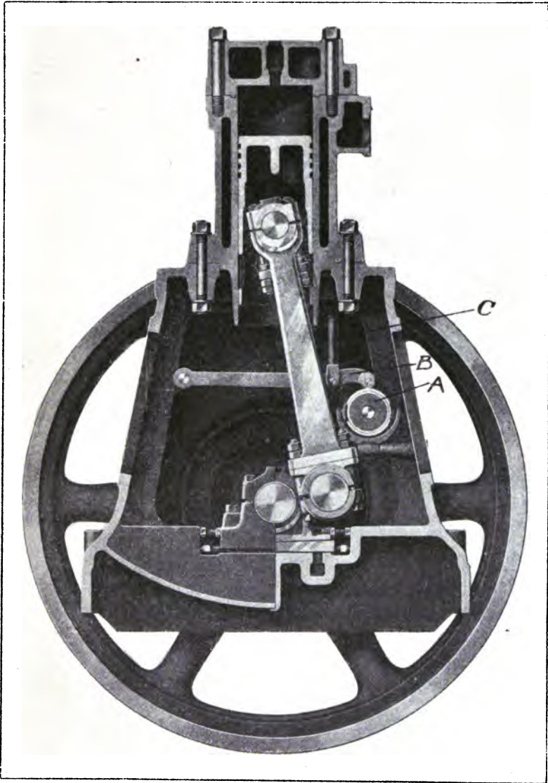
FIG. 73.—Diesel Engine.
